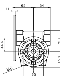
Gearbox Dimensions
